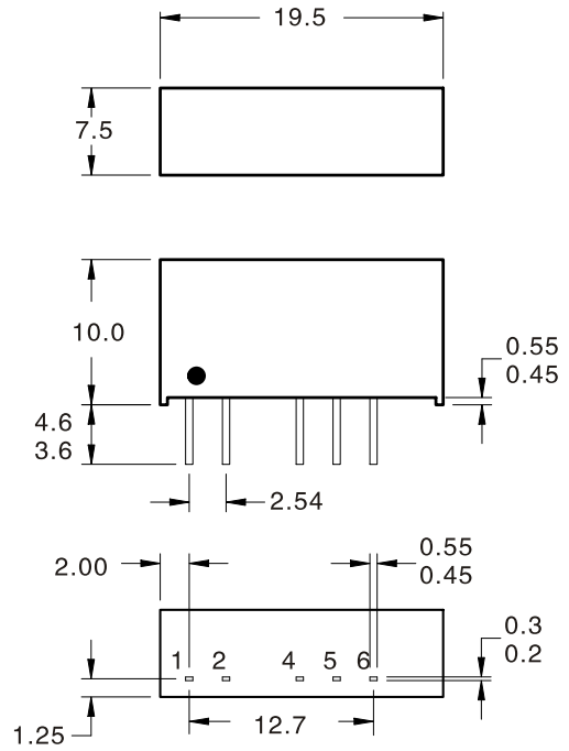
SIP PACKAGE
